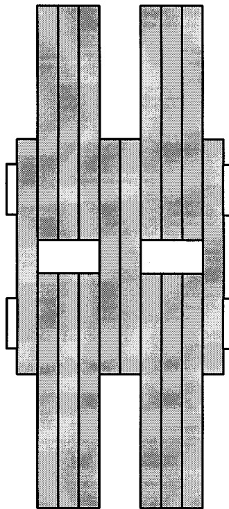
BH-7036 BL Chain 4 x 6 Lacing 1" Pitch
