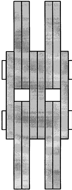
BH-7035 BL Chain 4 x 4 Lacing 1" Pitch
