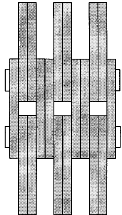
BH-7037 BL Chain 6 x 6 Lacing 1" Pitch
